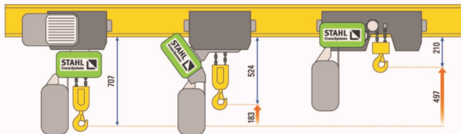
Standard headroom
